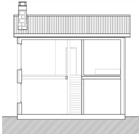
Sections
