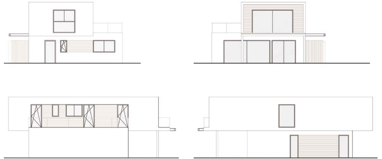
Elevations
