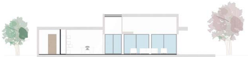
B-B' section
