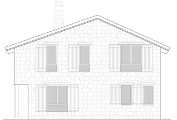
Northwest elevation
